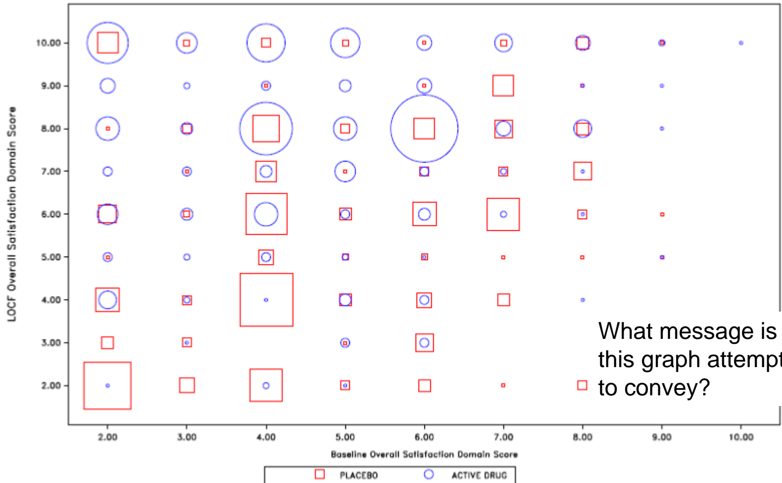
Plot of Each Subject's Baseline and LOCF Scores IEEF – Overall Satisfaction Domain Score
